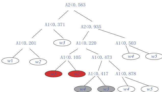
Fig. 3. Nonmonotonic decision tree trained with CART, where two pairs of rules are not monotonically consistent.
