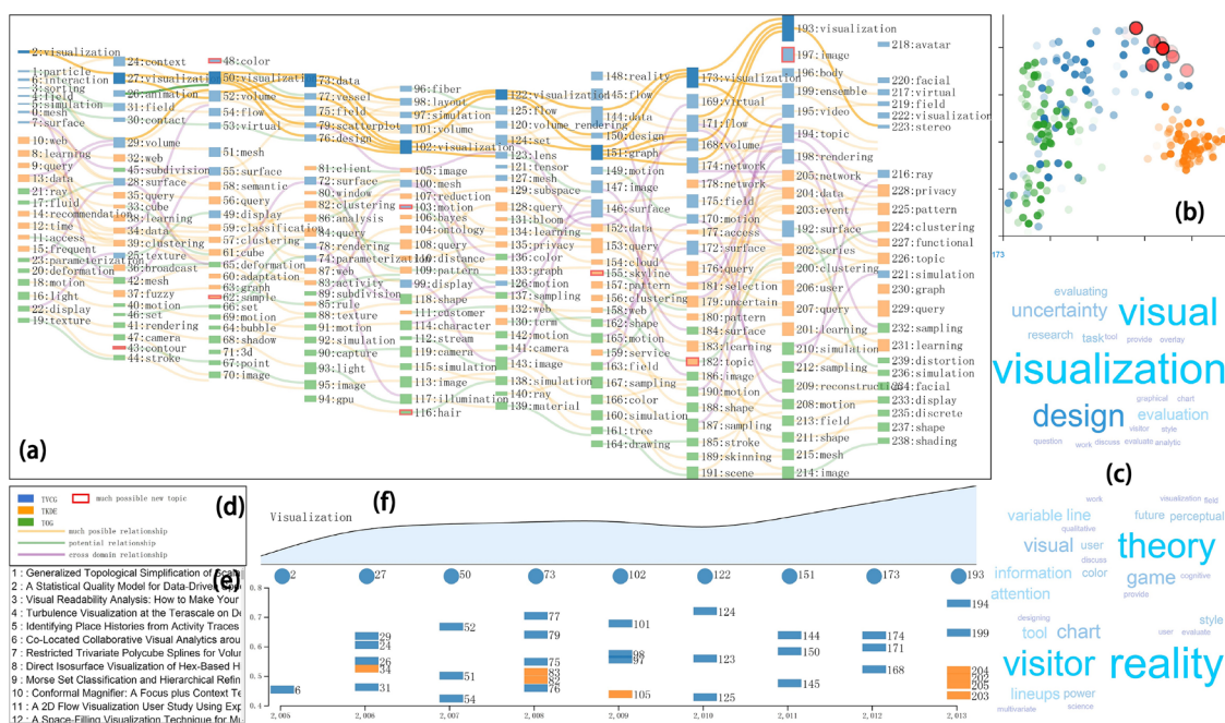
Fig. 1 Overview of the visualization tools. a sankey diagram presenting the topics for 10 years; b scatter plot showing the topics in 2D space; c word cloud of the selected topics and subtopics; d legend; e titles of the papers on the selected topics; and f stream diagram illustrating the topic trend with a scatterplot to show topic similarities
